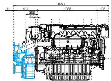
With YX75 gearbox / Right side view
