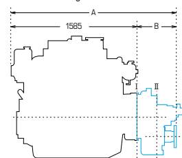
With YX120L gearbox / Left side view
