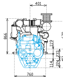
With YXH160 gearbox / Rear view
